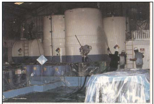
Figure 3. Tanks can be steam-cleaned, pressure washed or mechanically cleaned to customer's specifications. State of the art equipment is used to clean tanks from 200 to tanks in excess of 100,000 gallons.
